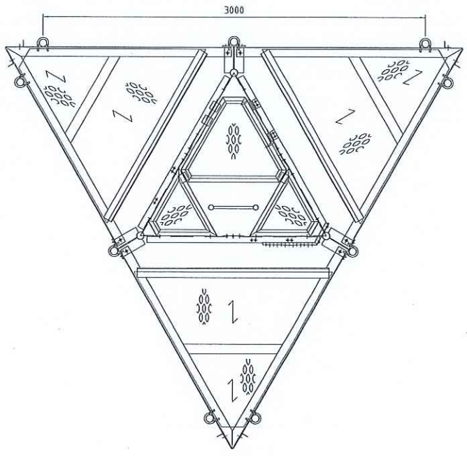
PLAN VIEW OF HEADFRAME
